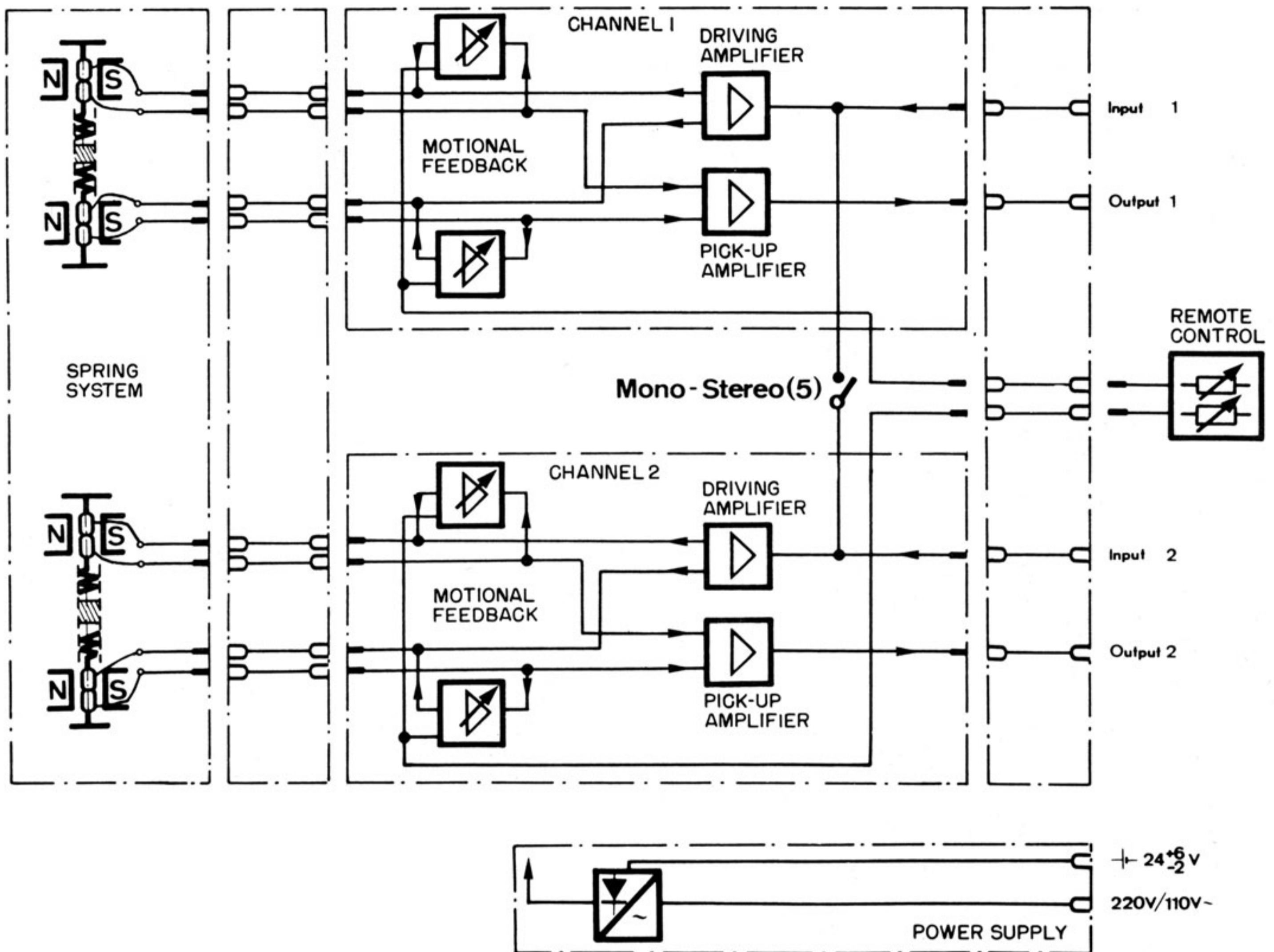
Figure 3 Block Diagram BX 20E
