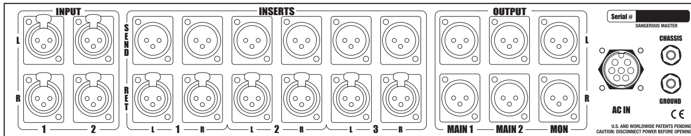
DANGEROUS MASTER REAR PANEL
