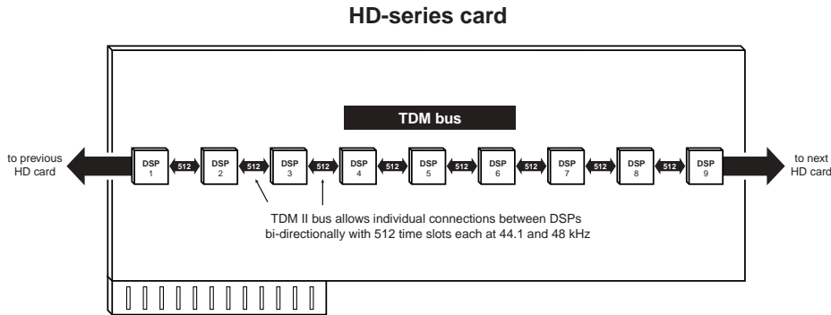
Figure 50. TDM bus on Pro Tools HD-series hardware
