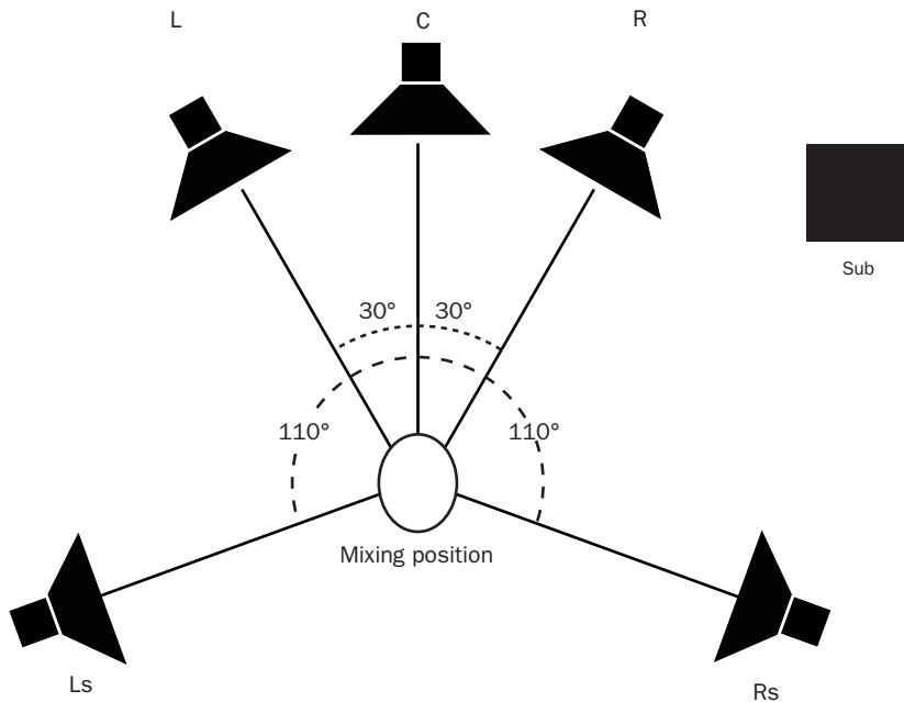
Figure 34. Example of speaker arrangement for 5.1 mixing and monitoring (SMPTE specification). Sub placement is variable, while all other speakers should be as close to the suggested angles as possible.
