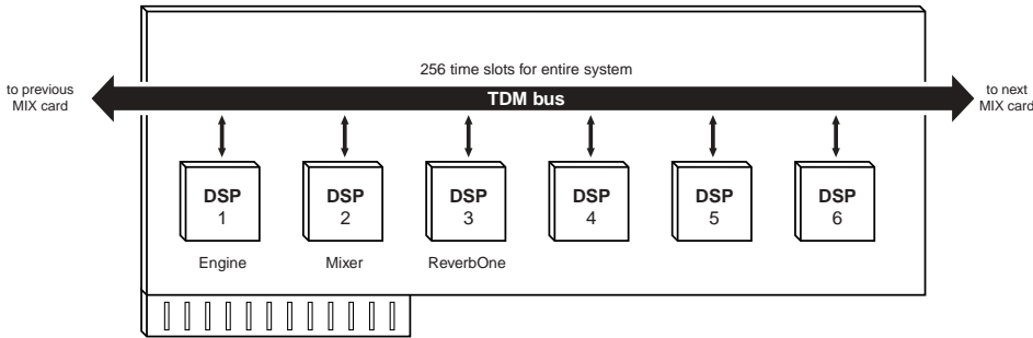
Figure 49. TDM bus on Pro Tools MIX-series hardware
