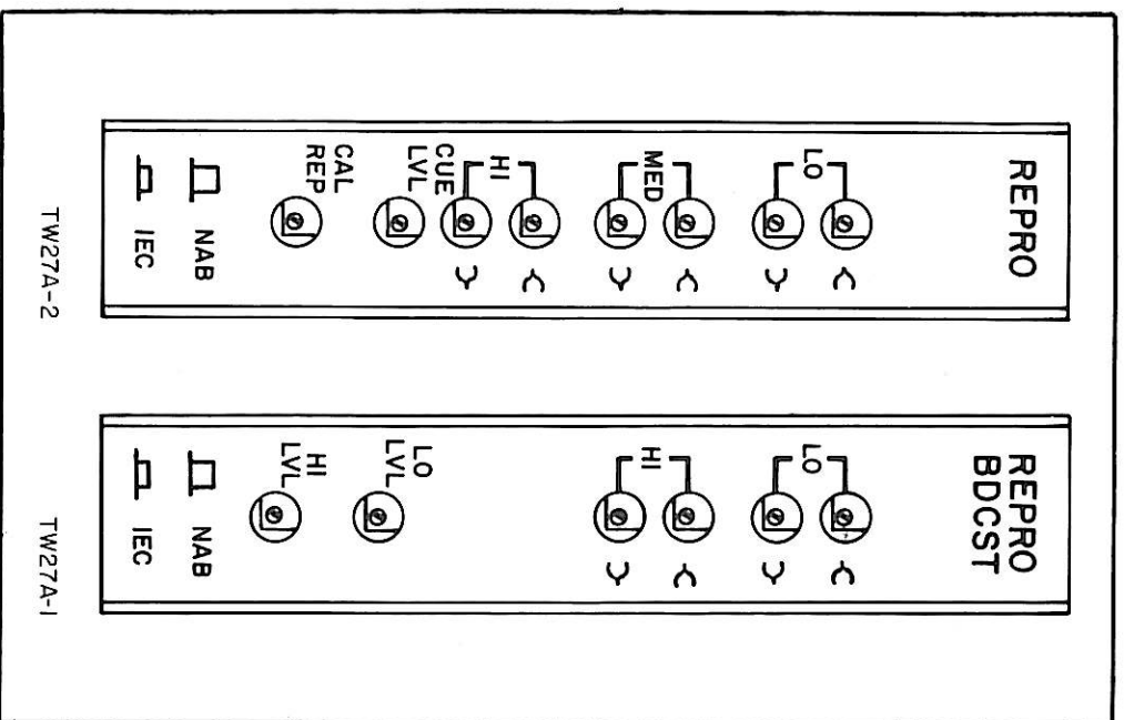
Figure 7-6 Repro Card Adjustment
