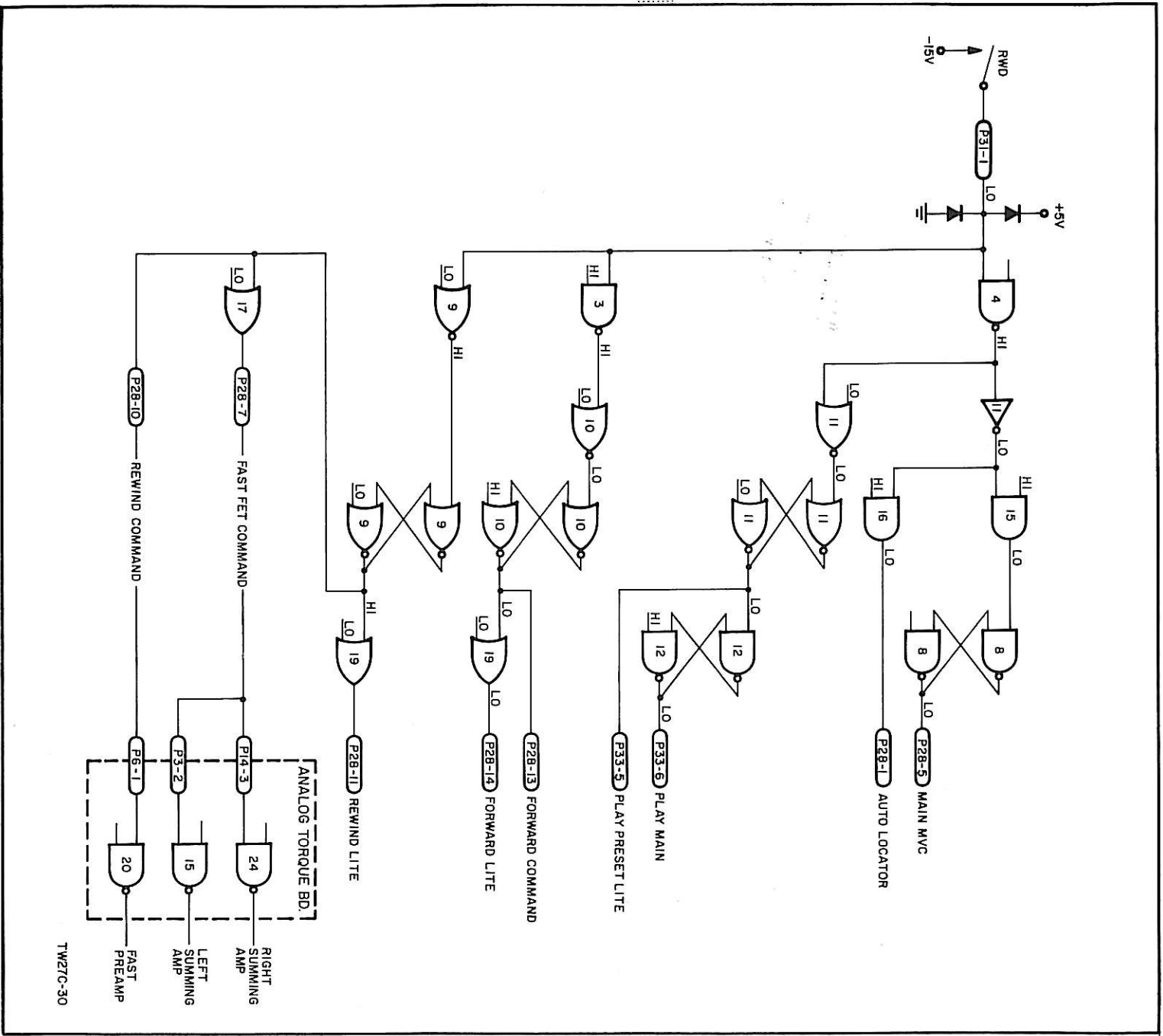
Figure 3-5 Rewind Command
