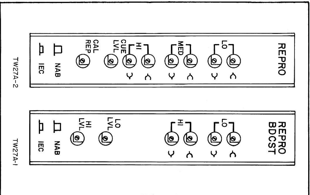
Figure 7-6 Repro Card Adjustment
