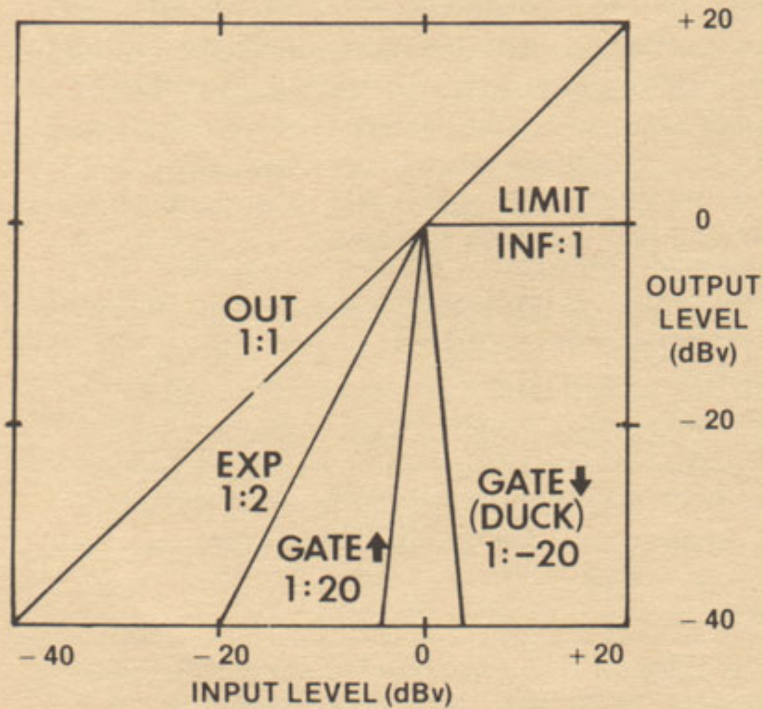
FIGURE 1 BASIC TRANSFER CHARACTERISTICS (INTERNAL DETECT MODE) THRESHOLD: 0dBv RANGE: 60dB OUTPUT: 0dB
