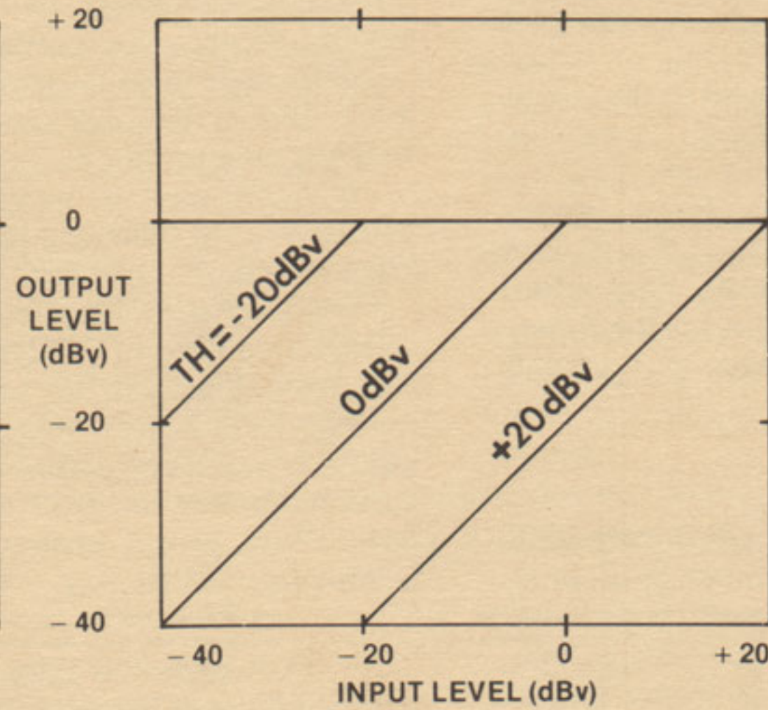
FIGURE 2 EFFECT OF THRESHOLD IN LIMIT MODE DETECT MODE: INTERNAL OUTPUT: 0dB RANGE: NOT APPLICABLE
