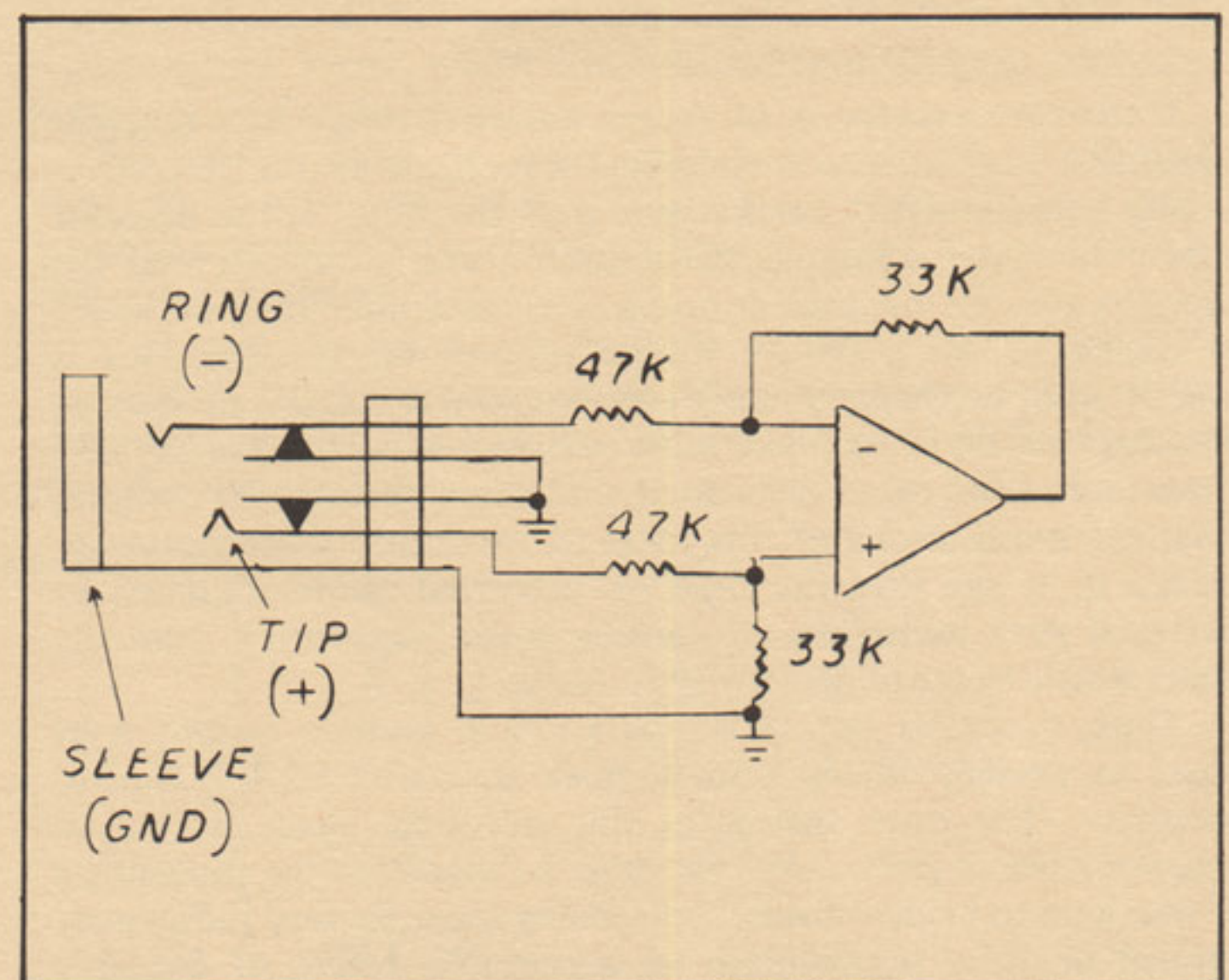
FIGURE 3 INPUT & EXT INPUT CONNECTOR CONFIGURATION (BALANCED)
